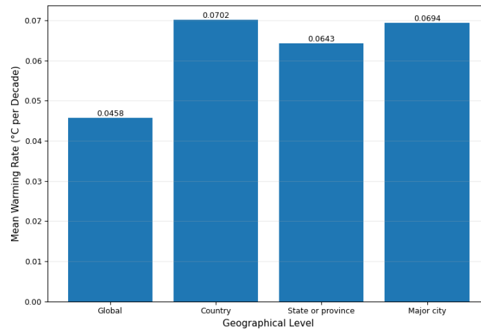
Figure 4. Mean Warming Rates Across Geographical Levels
