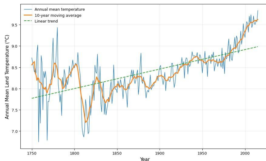
Figure 1. Annual Global Land Temperature Trend
